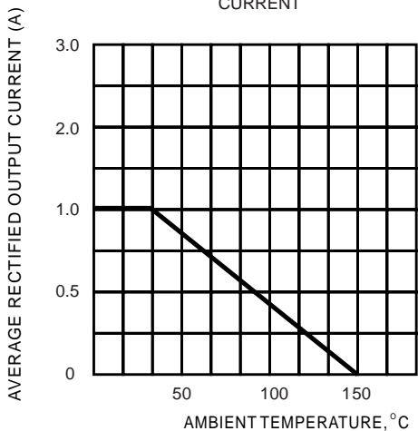
FIG. 2 DERATING CURVE FOR OUTPUT RECTIFIED CURRENT
