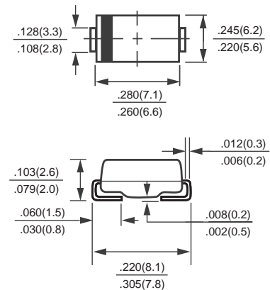
SMC(DO-214AB)
