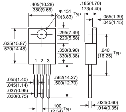
TO-220AB
