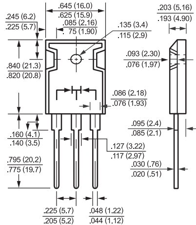
TO-3P
